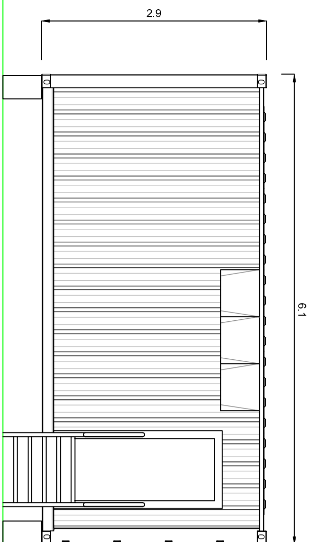
Front Elevation Typical Inverter
