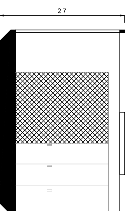
Section A - A Typical Transformer
