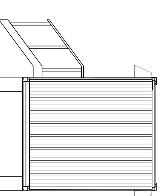
Side Elevation (Solid) Typical Inverter
